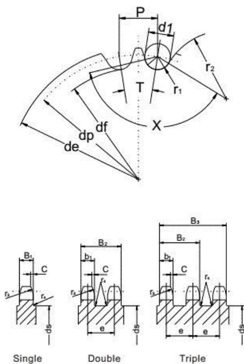
Single Double Triple Dimensions in mm
